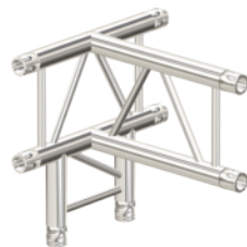
CODE:M32-4W-V 4WAY VERTICAL L500 W500 H500(mm)
