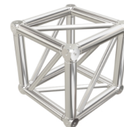
CODE: H44P BOX BOX CORNER M12 BOLT L400 W400 H400(mm)
