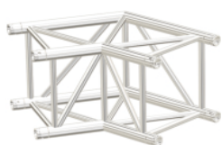
CODE: H44-2W-120 2WAY 120 degree L500 W500 H400(mm)
