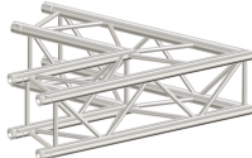
CODE: M34P-2W-60 2WAY 60 degree L290 W1000 H1000(mm)
