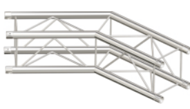
CODE: D24-2W-135 2WAY 135 degree L500 W500 H220(mm)
