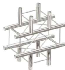
CODE: D24-4W-CROSS 4WAY CROSS L500 W500 H220(mm)
