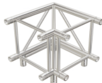
CODE: H44-3W-C30 3WAY C30 L500 W500 H400(mm)
