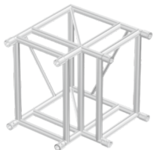
90° 2WAY CODE H7652-2W-90 L780 W780 H780(mm)
