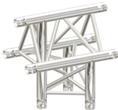
CODE:M33-3W-T39 3WAY T39 L257 W500 H500(mm)
