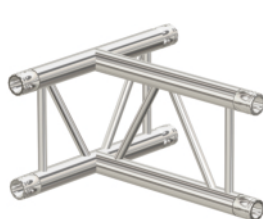
CODE:M32-T2V 3WAY VERTICAL L290 W500 H500(mm)
