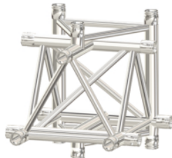
CODE: H43-5W-T51 5WAY T51 L500 W500 H500(mm)
