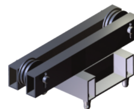
H7652-Top H7652 Top section for electrical chain hoist, hand chain hoist
