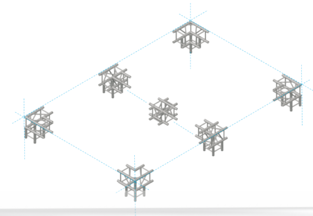
CODE: M34 BOOK BOOK CORNER L290 W290 H290(mm)
