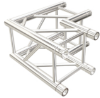
CODE: M34P-2W-90 2WAY 90 degree L290 W500 H500(mm)
