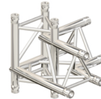
CODE:M33-4W-C44 4WAY C44 L500 W500 H500(mm)
