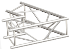
CODE: H44-2W-60 2WAY 60 degree L1000 W1000 H400(mm)
