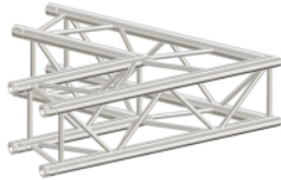
CODE: M34-2W-60 2WAY 60 degree L290 W1000 H1000(mm)
