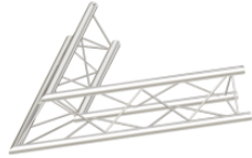
CODE: D23-2W-60 2WAY 60 degree L1000 W1000 H194(mm)
