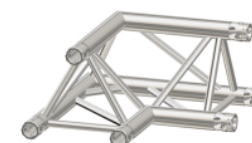
CODE:M33-2W-135 2WAY 135 degree L257 W500 H500(mm)
