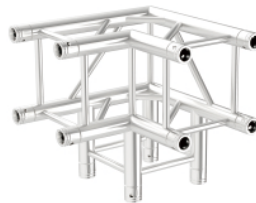
CODE: M34-3W-C30 3WAY C30 L500 W500 H500(mm)
