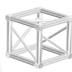
CODE: H44 BOX BOX CORNER M12 BOLT L400 W400 H400(mm)
