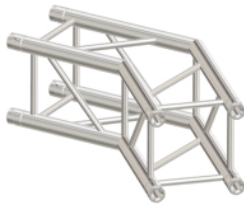
CODE: M34-2W-135 2WAY 135 degree L290 W500 H500(mm)
