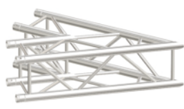
CODE: M34P-2W-45 2WAY 45 degree L290 W1000 H1000(mm)
