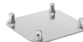
CODE: H44P BASE BASE PLATE L420 W420 H080(mm)
