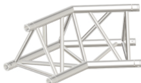
CODE: H43-2W-135 2WAY 135 degree L500 W500 H353(mm)
