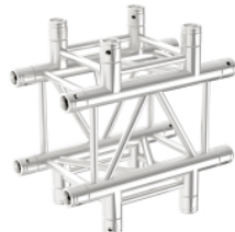
CODE: M34P-CROSS 4WAY CROSS L290 W500 H500(mm)
