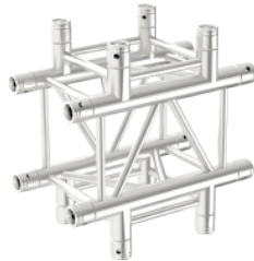
CODE: M34-CROSS-T41 4WAY CROSS L290 W500 H500(mm)
