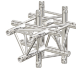
CODE:M33-5W-C51 5WAY C51 L500 W500 H500(mm)
