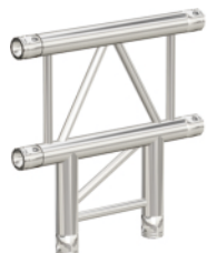
CODE:M32-T2H 3WAY HORIZONTAL L500 W050 H500(mm)
