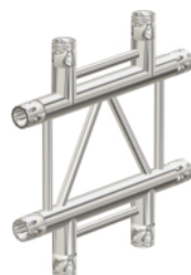
CODE:M32-CROSS-H CROSS HORIZONTAL L050 W500 H500(mm)
