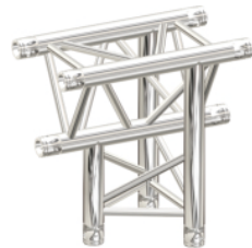
CODE:M33-3W-T38 3WAY T38 L290 W500 H500(mm)
