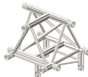
CODE: H43-4W-T43 4WAY T43 L400 W500 H500(mm)
