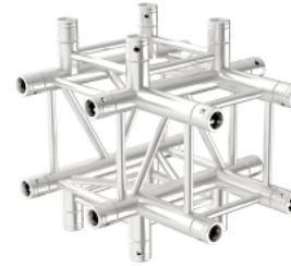
CODE: M34-5W 5WAY 90 degree L500 W500 H500(mm)
