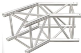
CODE: H44-2W-135 2WAY 135 degree L500 W500 H400(mm)
