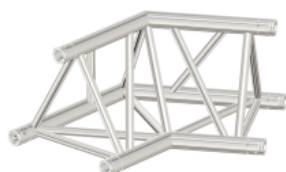
CODE: H43-2W-120 2WAY 120 degree L500 W500 H353(mm)
